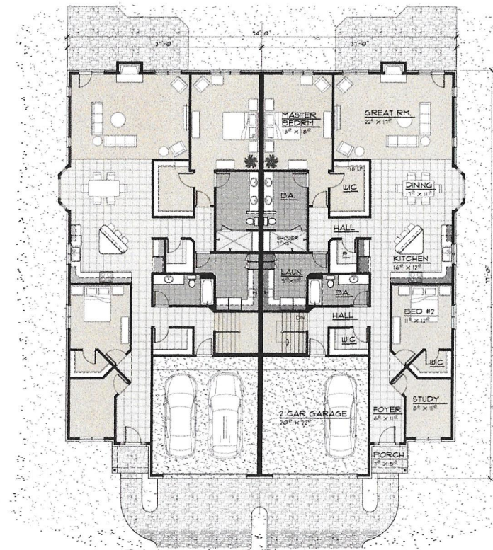
RANCH FLOOR PLAN
