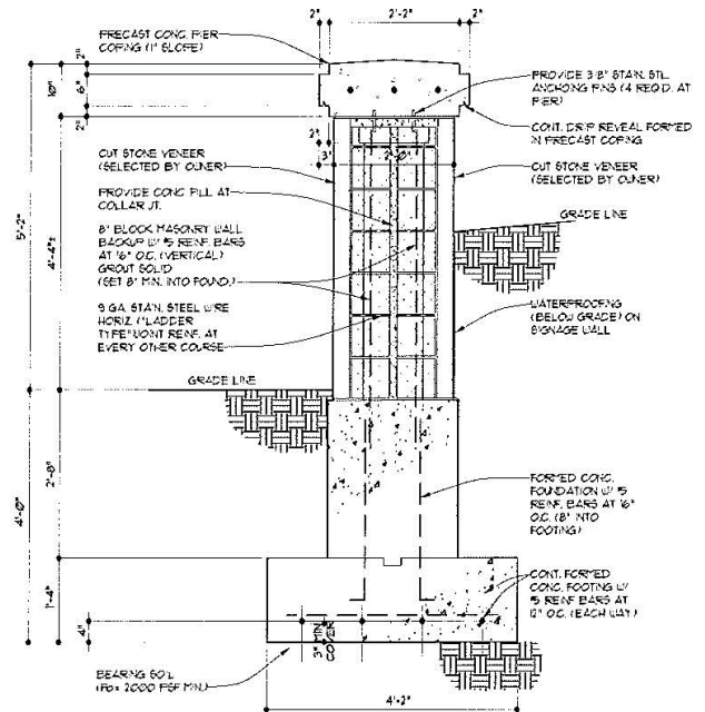
SECTION THRU WALL PIER SCALE: 3/4\" = 1'-0\"
