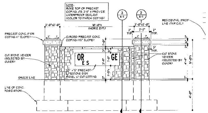
FRONT OF WALL ELEVATION SCALE: 1/2\" = 1'-0\"
