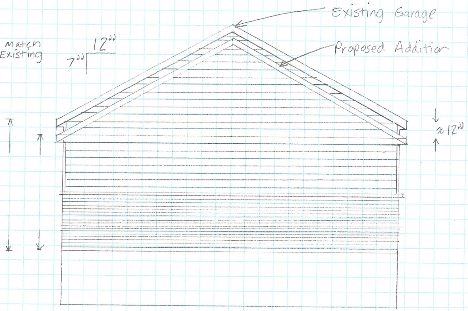
Proposed SOUTH ELEVATION
