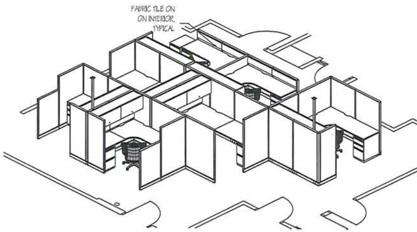
PERSPECTIVE VIEW B
